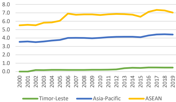
▶ Figure 8. CO2 emissions, 2000-2019, Timor Leste, ASEAN and Asia-Pacific (metric tonnes per capita)
