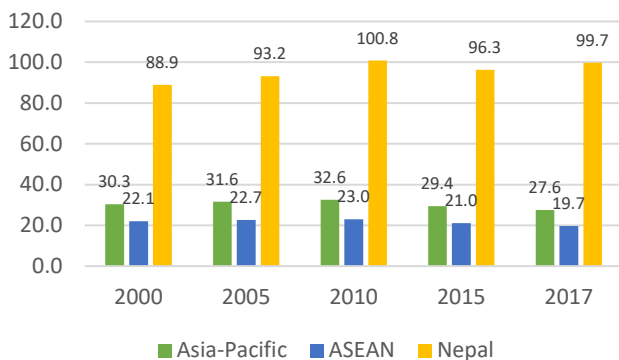
► Figure 9. Air quality PM 2.5 emissions, 2000-2017, Nepal, ASEAN and Asia-Pacific (micrograms per cubic metre)
