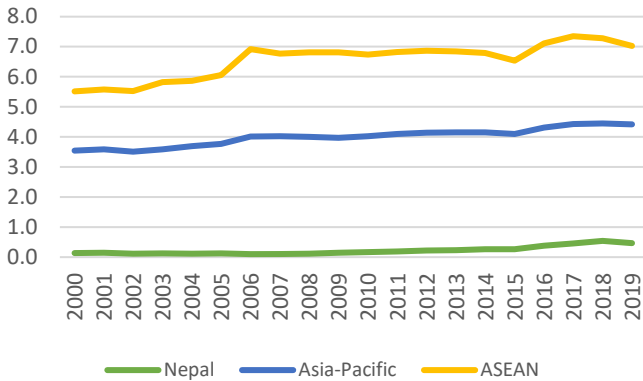
► Figure 8. CO2 emissions, 2000-2019, Nepal, ASEAN and Asia-Pacific (metric tonnes per capita)
