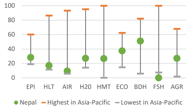
► Figure 5. Environmental performance index and selected indicators, Nepal and Asia-Pacific, 2022
