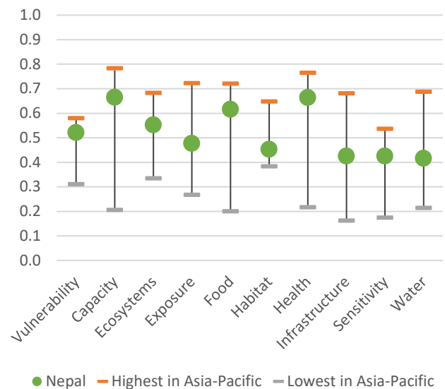
► Figure 10. Notre Dame Global Adaptation Index, Vulnerability and composite indicators, 2020, Nepal, Asia-Pacific (index score)
