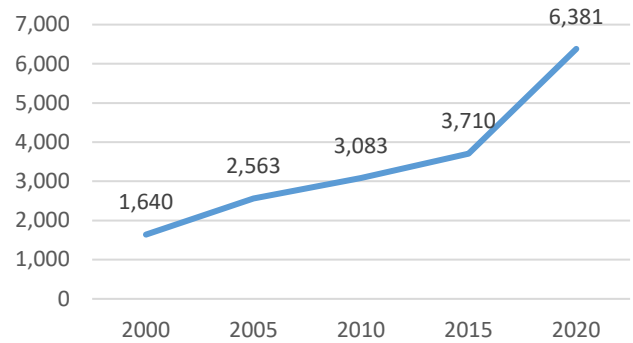
► Figure 12. Total renewable energy generation (GWh), 2000-2020
