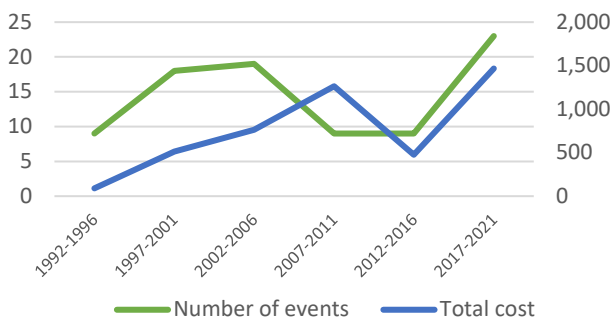
► Figure 11. Number of natural disasters (LHS) and total cost of natural disasters (RHS - US$ million) per 5-year period, 1992-2021
