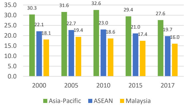
► Figure 9. Air quality PM 2.5 emissions, 2000-2017, Malaysia, ASEAN and Asia-Pacific (micrograms per cubic metre)
