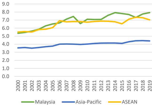
► Figure 8. CO2 emissions, 2000-2019, Malaysia, ASEAN and Asia-Pacific (metric tonnes per capita)
