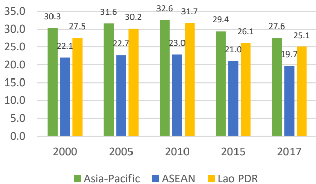
► Figure 9. Air quality PM 2.5 emissions, 2000-2017, Lao PDR, ASEAN and Asia-Pacific (micrograms per cubic metre)
