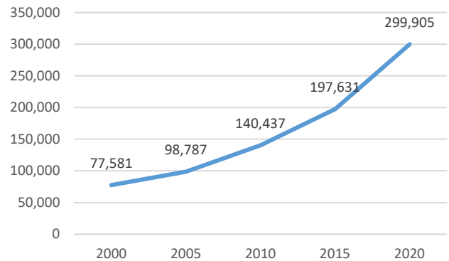
▶ Figure 12. Total renewable energy generation (GWh), 2000-2020
